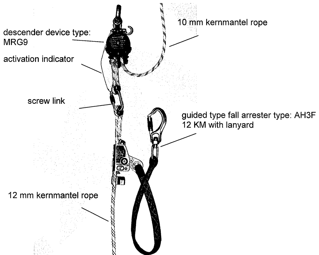
fig. 1: guided type fall arrester including a flexible anchor line type: FallArrescue
